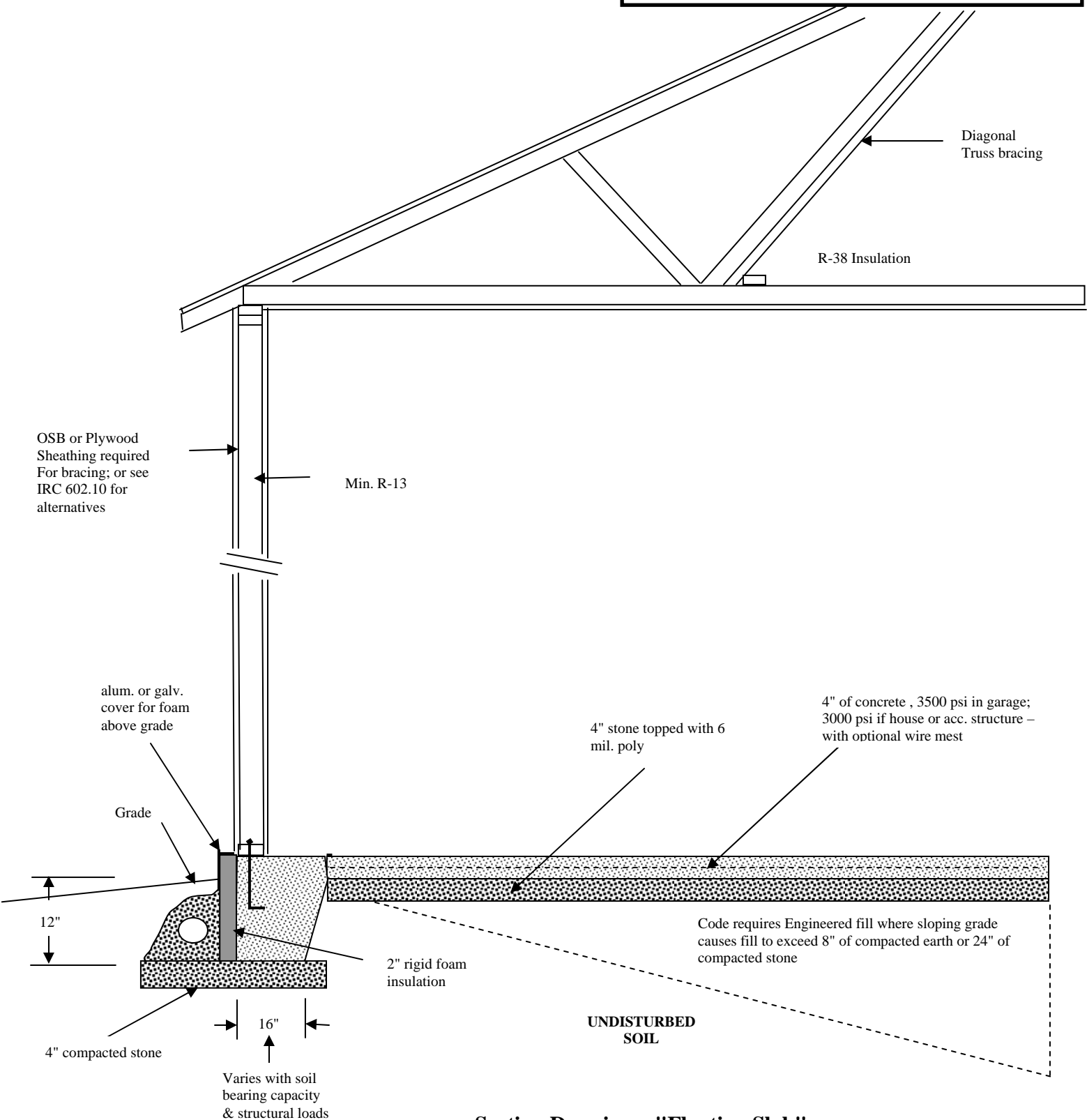
Section Drawing – "Floating Slab" Typical Turned-Down-Slab Alternative For House, Garage, Accessory Building Footer/Slab Construction. THIS STRUCTURE MUST BE HEATED TO 64° F. MINIMUM
